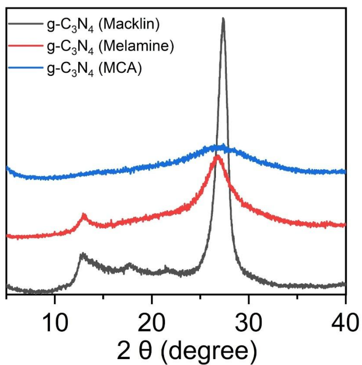
Figure 3. X-ray diffraction patterns of g-C 3 N 4 samples obtained in an inert atmosphere
