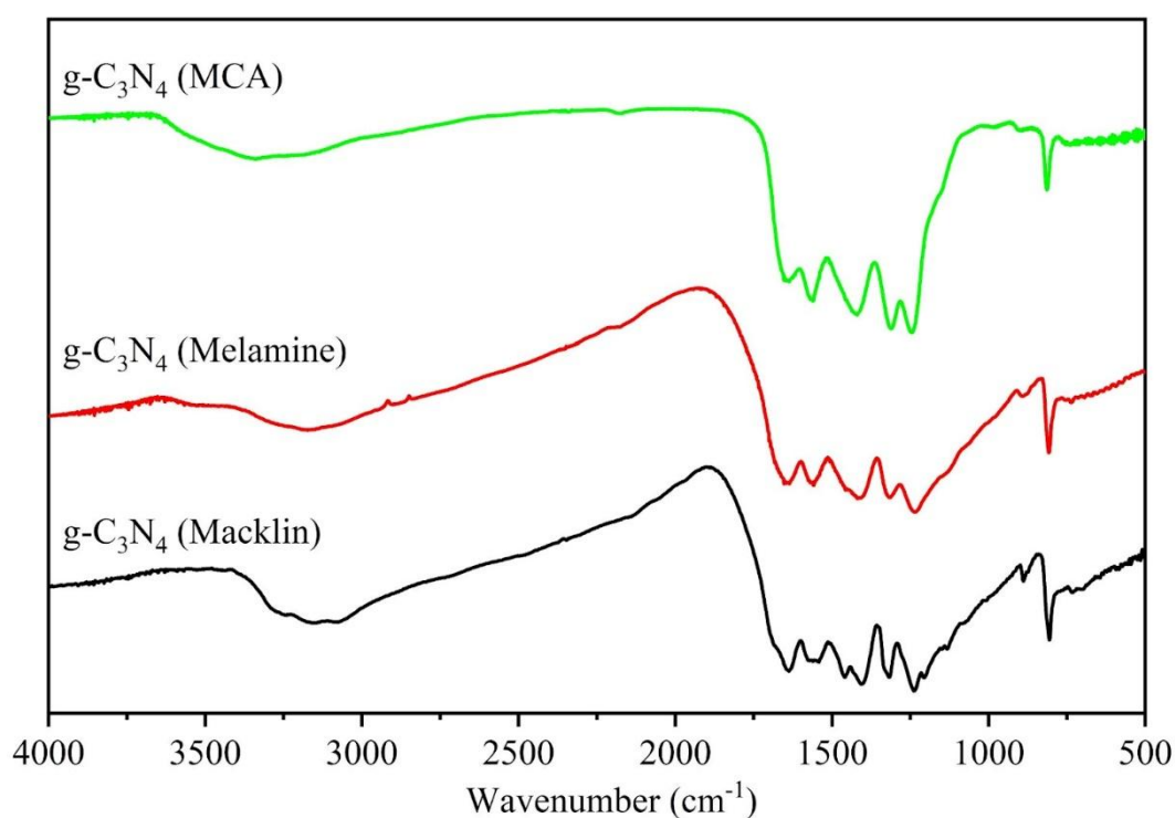
Figure 4. FTIR spectra of g-C 3 N 4 samples obtained in an inert atmosphere
